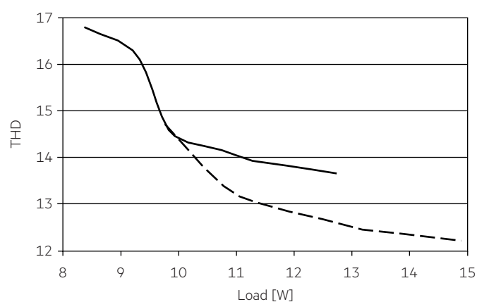
4.1.3 THD vs load
