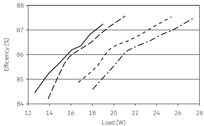
4.1.1 Efficiency vs load
